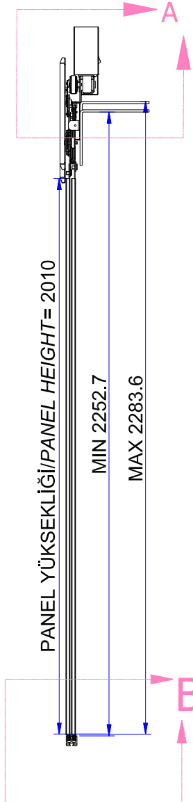
DETAY A DETAIL A
