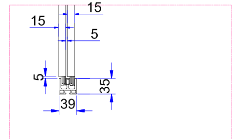
DETAIL B / DETAIL B
