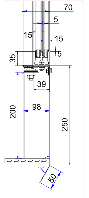
DETAIL B / DETAIL B
