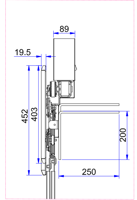
DETAY A DETAIL A
