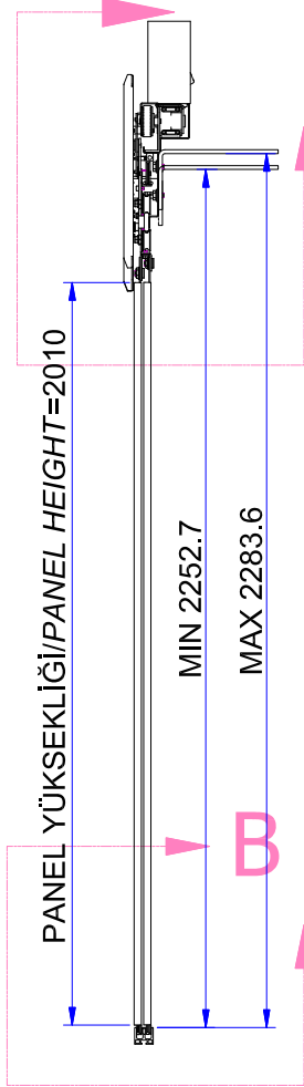
DETAIL A / DETAIL A
